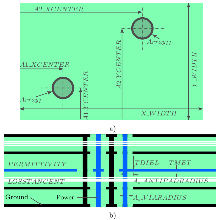
Figure 1: a) Top view of the PCB, b) side view of the PCB. The parameters are named as found in the data files. The array are numbered A1 , A2 , and additionally a VRM array is present on the board. The board number A1 or VRM is used as prefix for the array dependent parameter, e.g. via radius.
